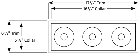
Three module
