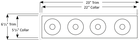
Four module
