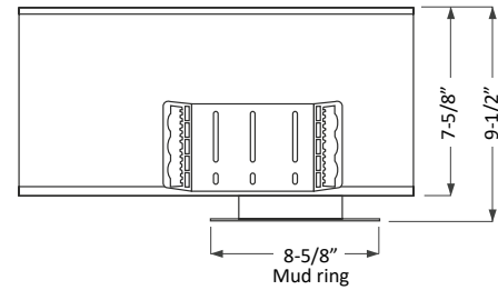
Mud ring
