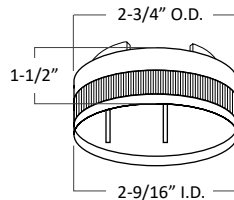
LED Holder
