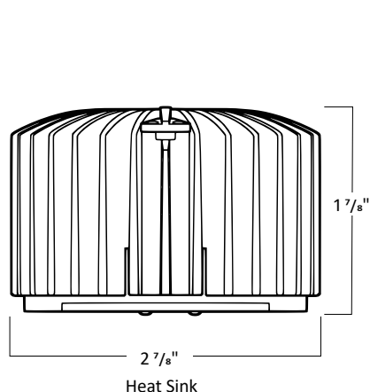
Heat Sink
