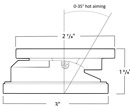
Adjustable Module Holder
